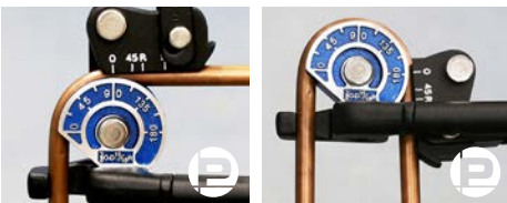
Doppel-Scharnier-Design
