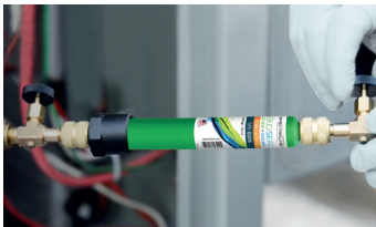
Charge inline with refrigerant
